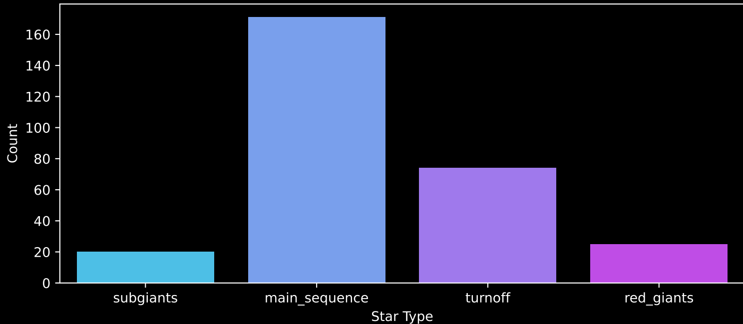
GALAH DR4 Field: [7028] Count plot of Star Type
