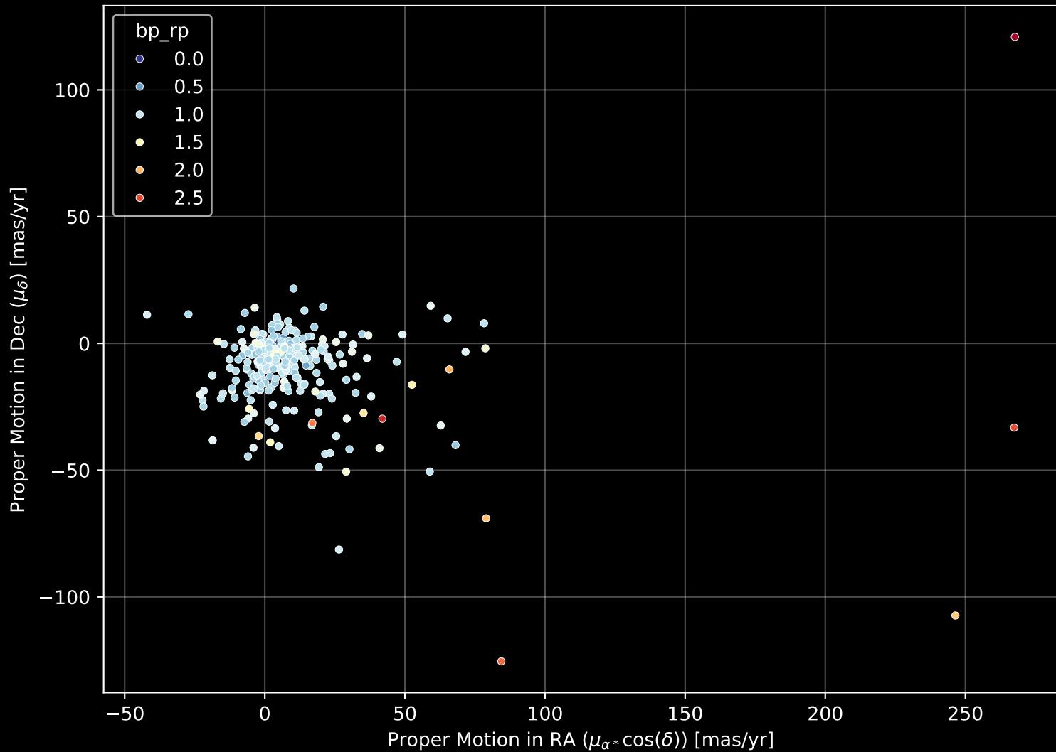
GALAH DR4 Field: [7028] Proper Motion Diagram (n= 290)
