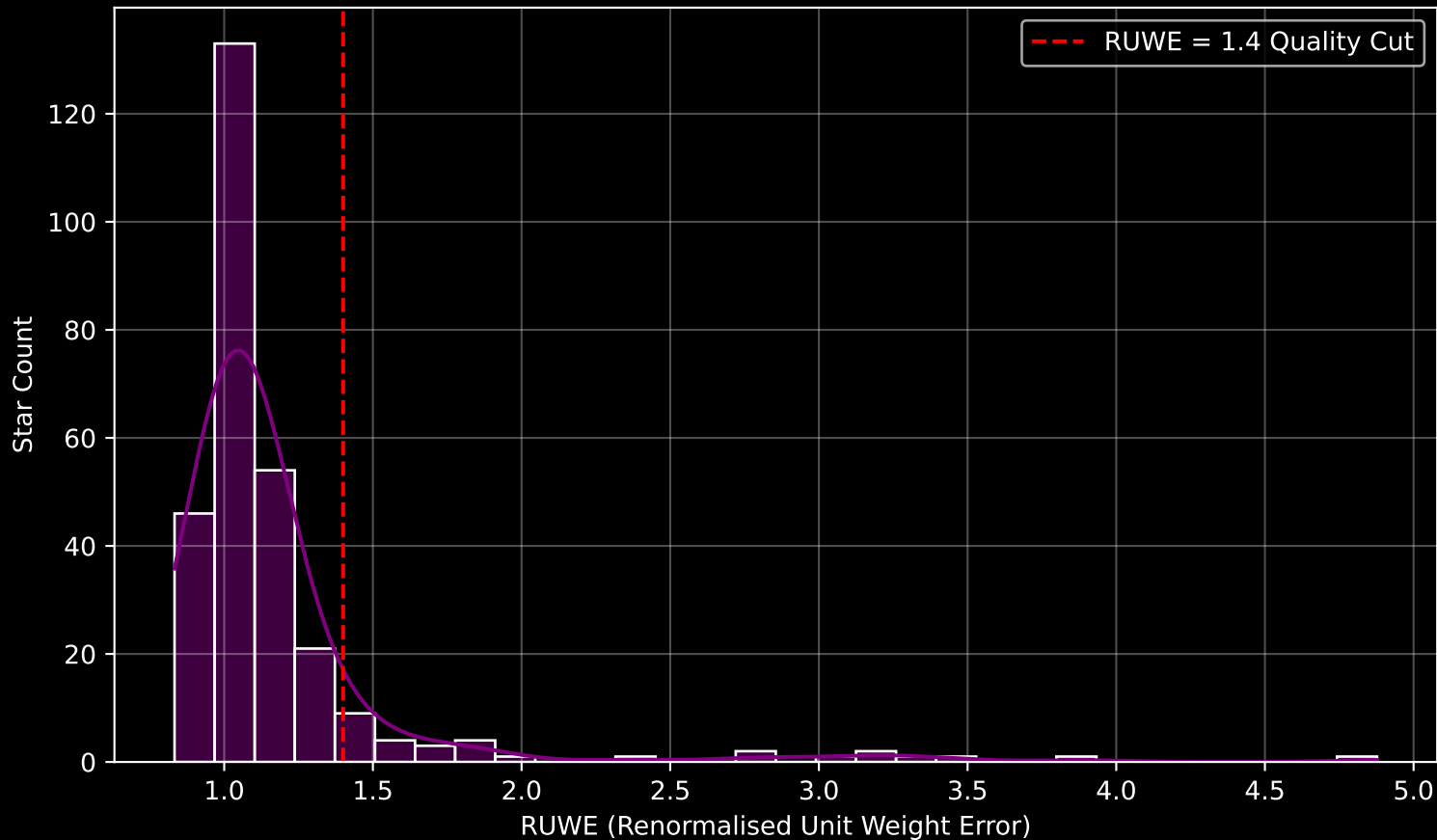
GALAH DR4 Field [7028] RUWE Distribution (n= 285)
