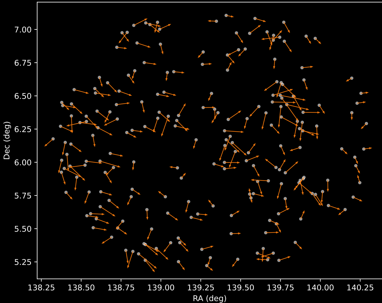
GALAH DR4 Cluster 2 Proper Motion Vectors (n=210)
